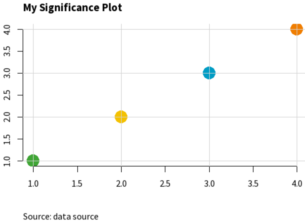
Figure 3: Scatter plot showing the base R styling implemented by set_signif_par() .
